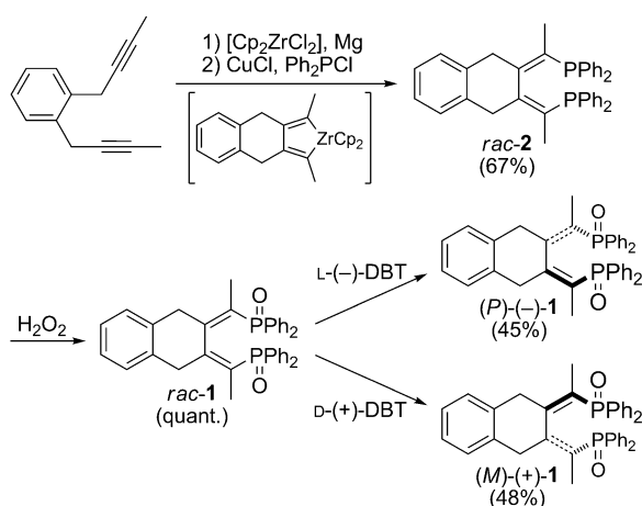
Scheme 2. Synthesis and chiral resolution of the atropisomeric chiral dienyI bisphosphine dioxide 1 .
